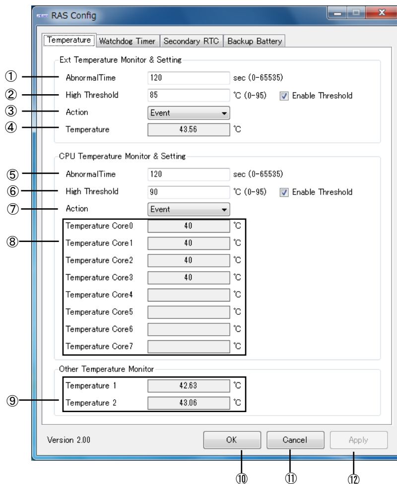
図 2-13-3-1. Temperature Configuration
