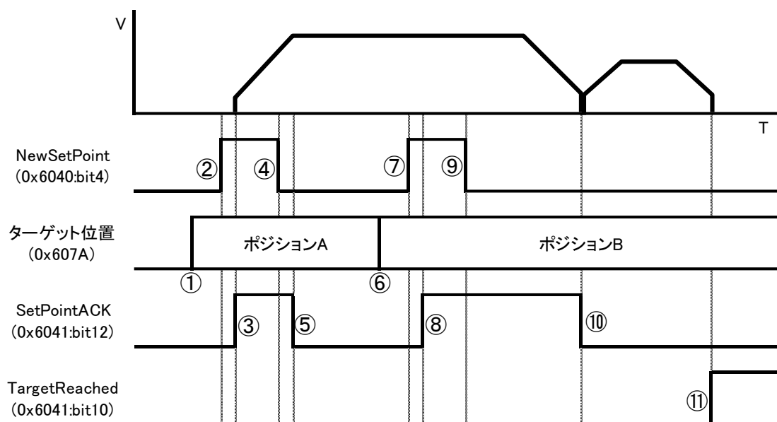
図 4-3-5-2 Set of Set-Points
