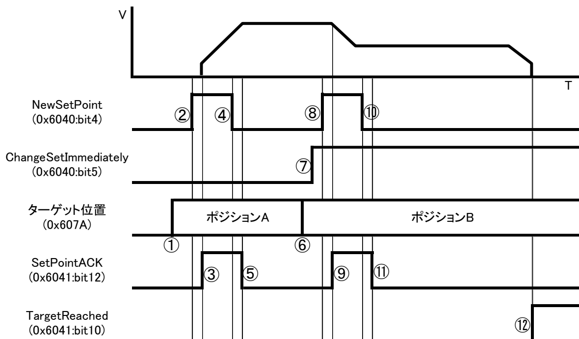
図 4-3-5-3 Single Set-Points
