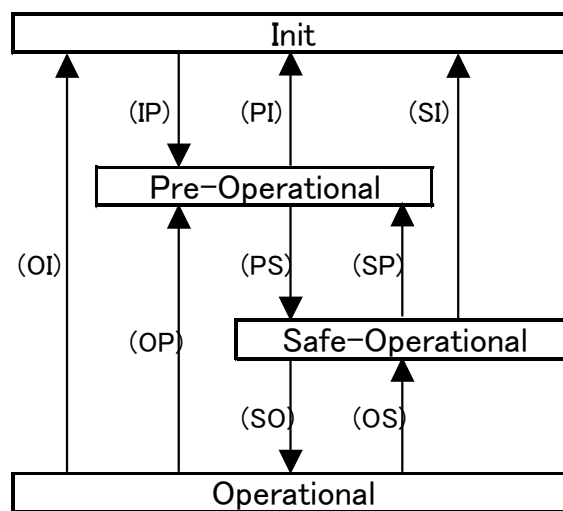
図 3-3-4-1 EtherCAT State Machine
