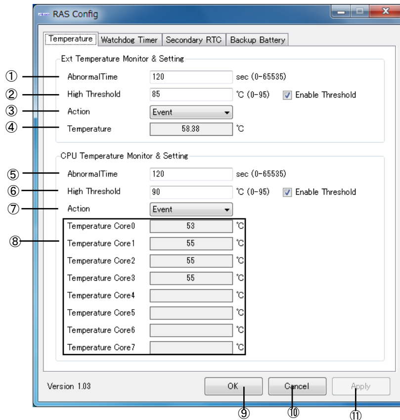
図 2-13-3-1. Temperature Configuration
