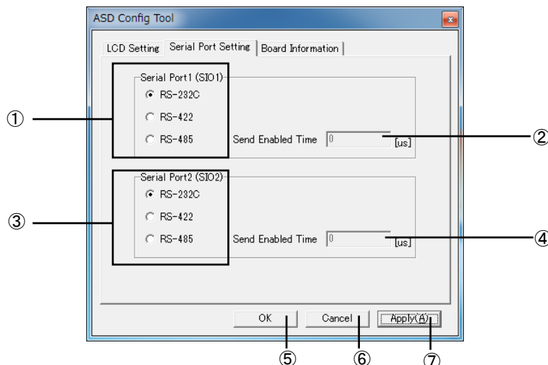
図 2-9-3-1. ASD Config – Serial Port Setting
