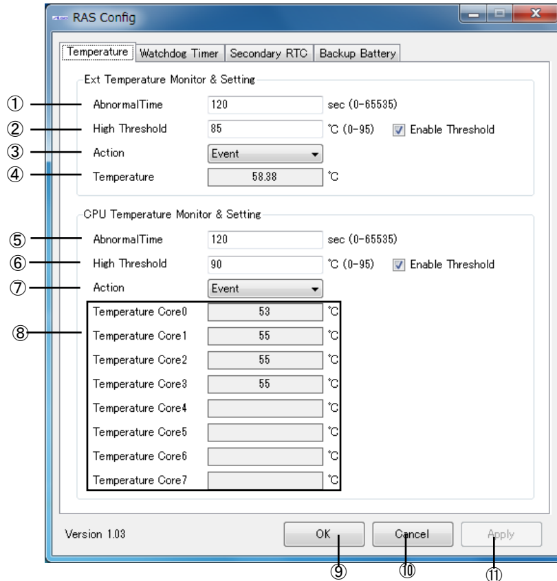
図 2-10-3-1. Temperature Configuration
