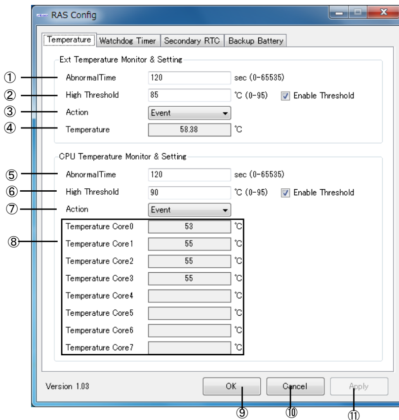
図 2-13-3-1. Temperature Configuration
