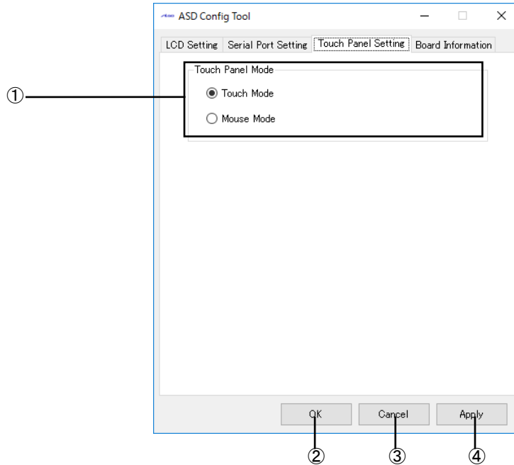
図 2-10-4-1. ASD Config – Touch Panel Setting
