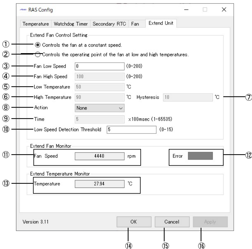
図 2-11-12-1. Extend Unit Configuration
