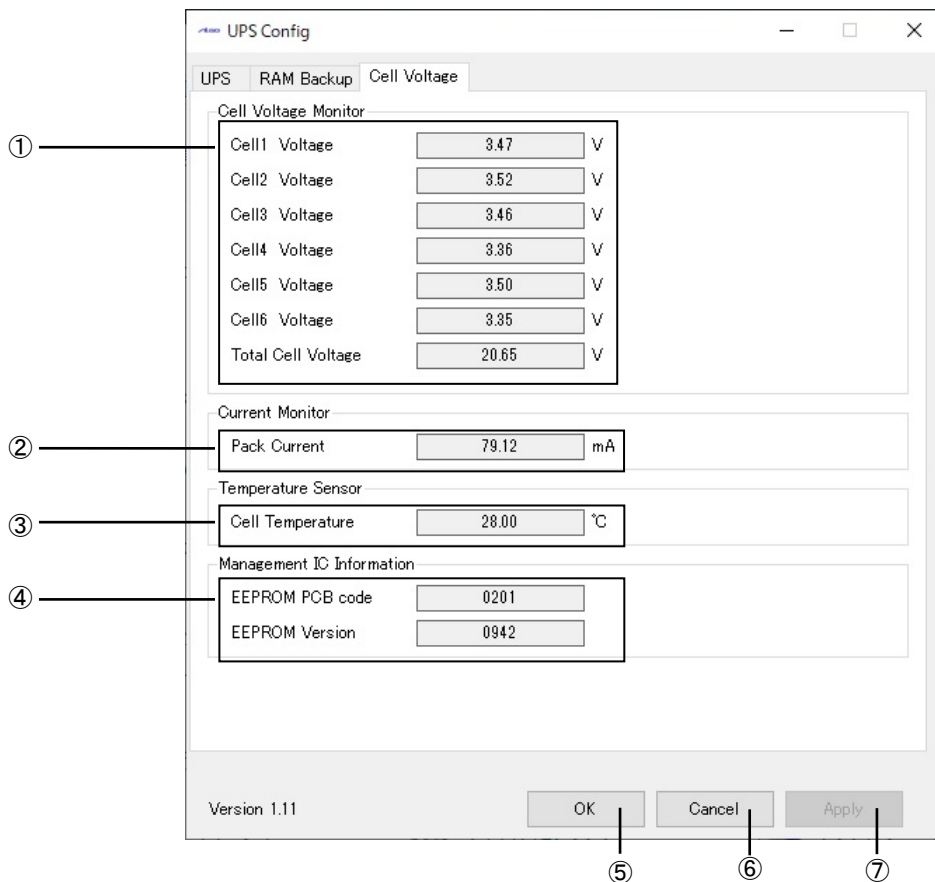
図 2-12-4-1. Cell Voltage
