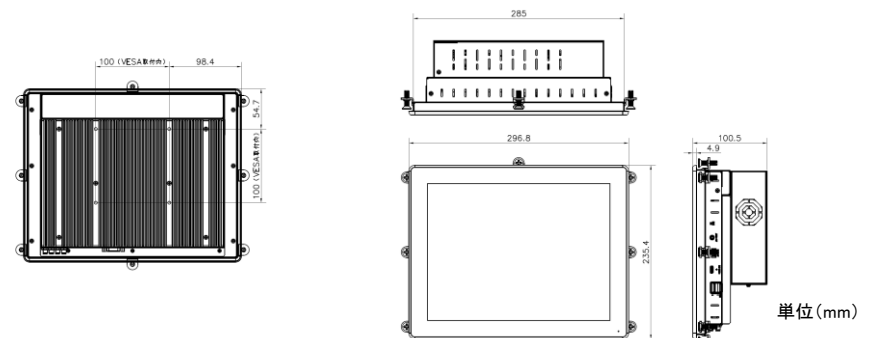
●NP6A-121xN/xS (拡張付)
