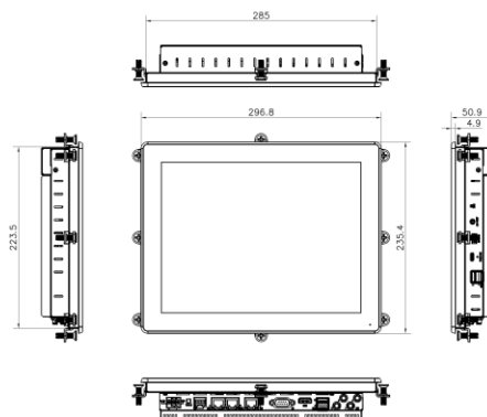
●NP6A-121xN/xS
