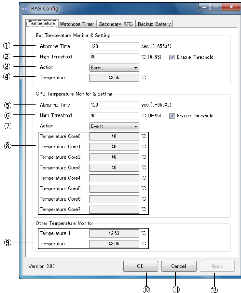
図 2-13-3-1. Temperature Configuration
